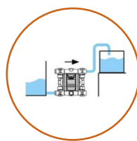
Positive Suction Head
